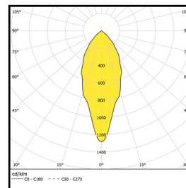
Flood 35 W, 39°
