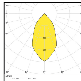
Flood 70 W, 54°
